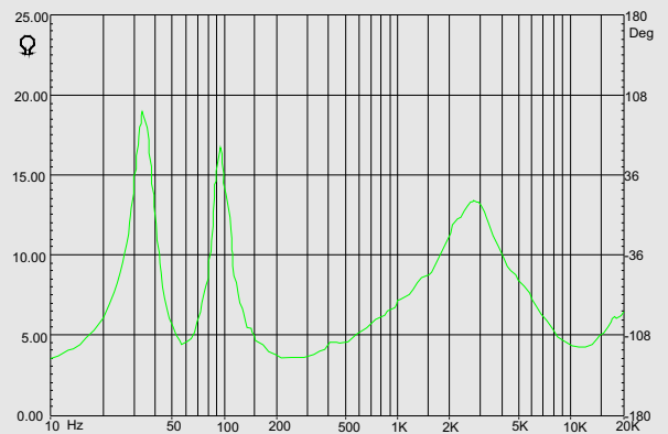
IMPEDANCE CURVE
