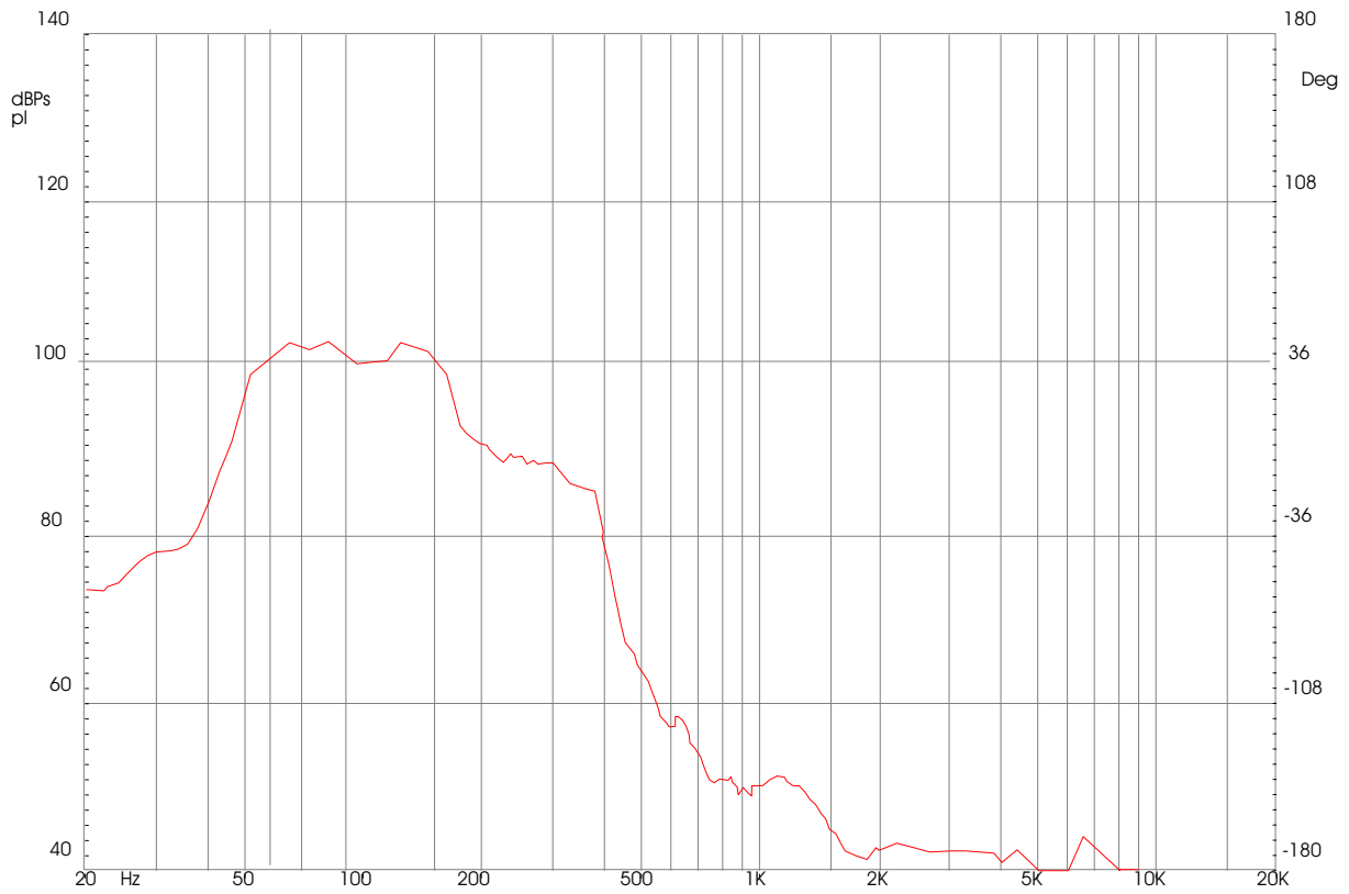
FREQUENCY RESPONSE
